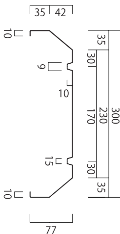
鼻隠しDX300
