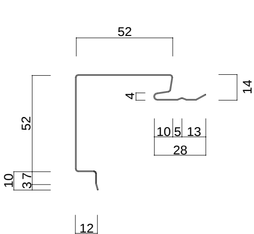
SPR105 (出隅) L = 2000 ~ 3000
