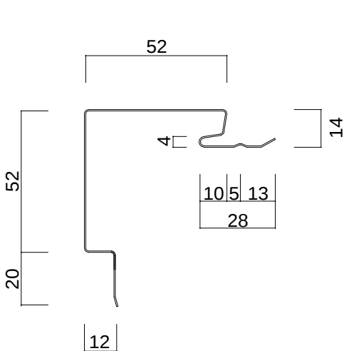
SPR116 (出隅) L = 2000 ~ 3000
