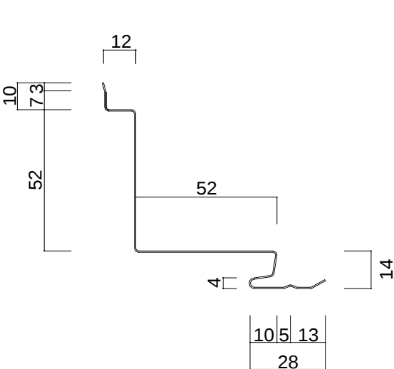
SPR105 (入隅) L = 2000 ~ 3000
