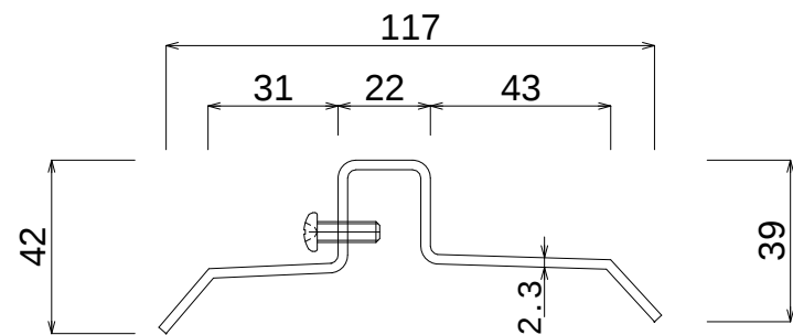
K R角ハゼ500 ( D 1 6 0 ) 吊子W = 3 0
