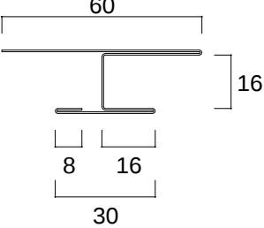
R S - 4 0 0 ( H型接続 ) L = 2 0 0 0 ~ 3 0 0 0
