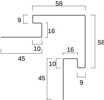
R S - 3 0 0 ( 横張用・出隅 ) L = 2 0 0 0 ~ 3 0 0 0
