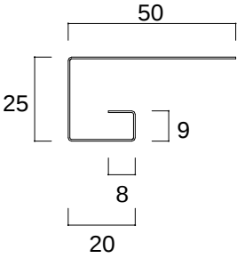
R S - 1 0 1 ( 廻り縁 ) L = 2 0 0 0 ~ 3 0 0 0
