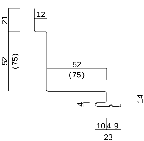
R S R - 3 0 4 ( 入 隅 ) L = 2 0 0 0 ~ 3 0 0 0
