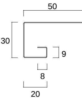
NK - 1 0 1 ( 廻り縁 ) L = 2 0 0 0 ~ 3 0 0 0
