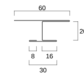
NK - 4 0 0 ( H型接続 ) L = 2 0 0 0 ~ 3 0 0 0
