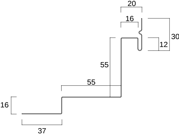
NKR - 3 0 4 ( 入 隅 ) L = 2 0 0 0 ~ 3 0 0 0
