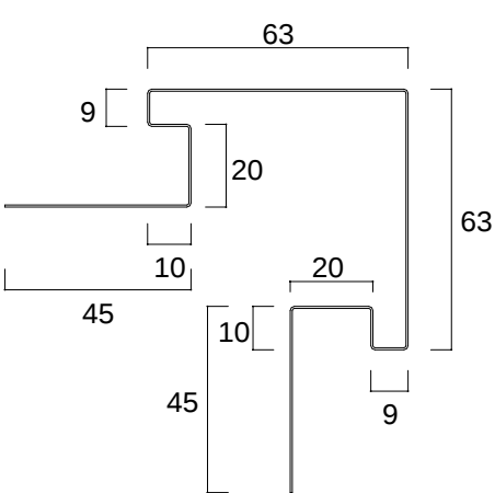
NK - 3 0 0 ( 横張用・出隅 ) L = 2 0 0 0 ~ 3 0 0 0
