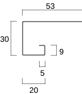
NKR - 1 0 1 ( 廻り縁 ) L = 2 0 0 0 ~ 3 0 0 0
