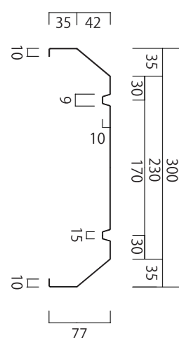
鼻隠しDX300
