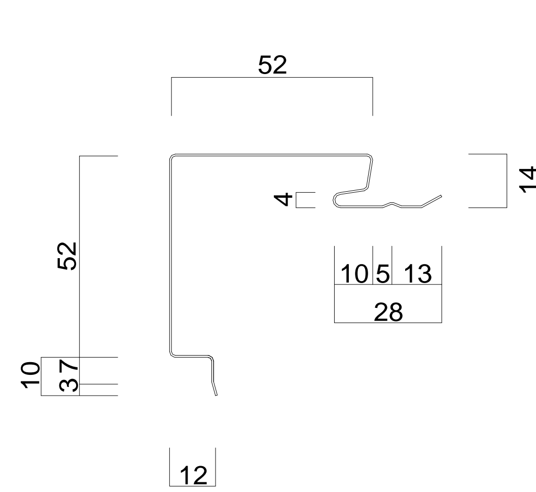
SPR105 (出隅) L = 2000 ~ 3000
