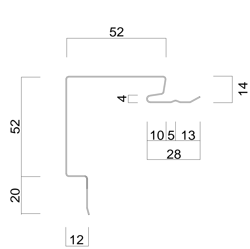
SPR116 (出隅) L = 2000 ~ 3000
