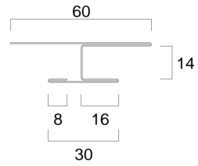
SP-400 (H型接続) L = 2000 ~ 3000
