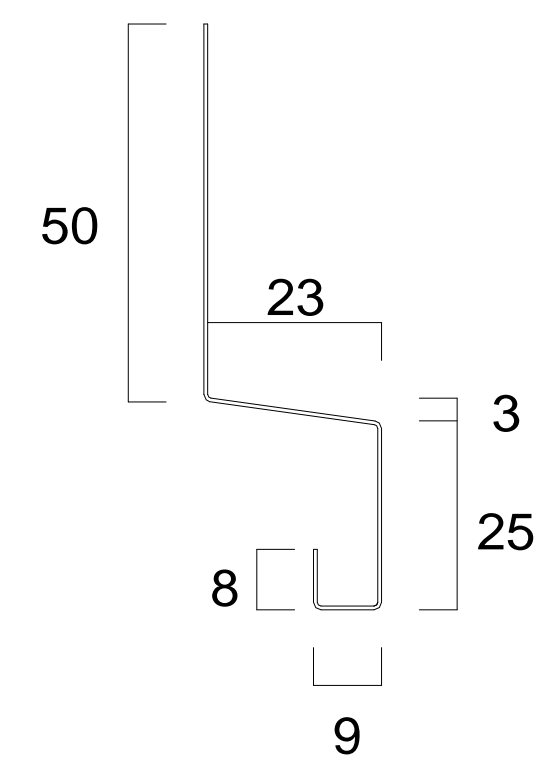
SP-202 (中間水切接続) L = 2000 ~ 3000
