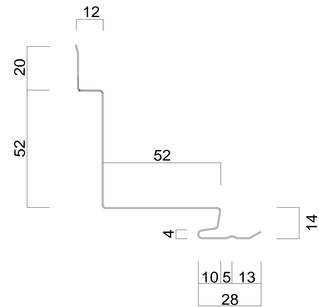
SPR116 (入隅) L = 2000 ~ 3000
