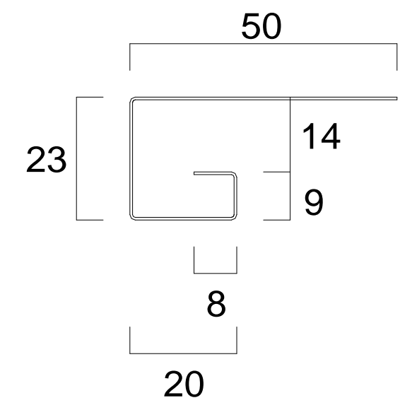
SP-101 (廻り縁) L = 2000 ~ 3000
