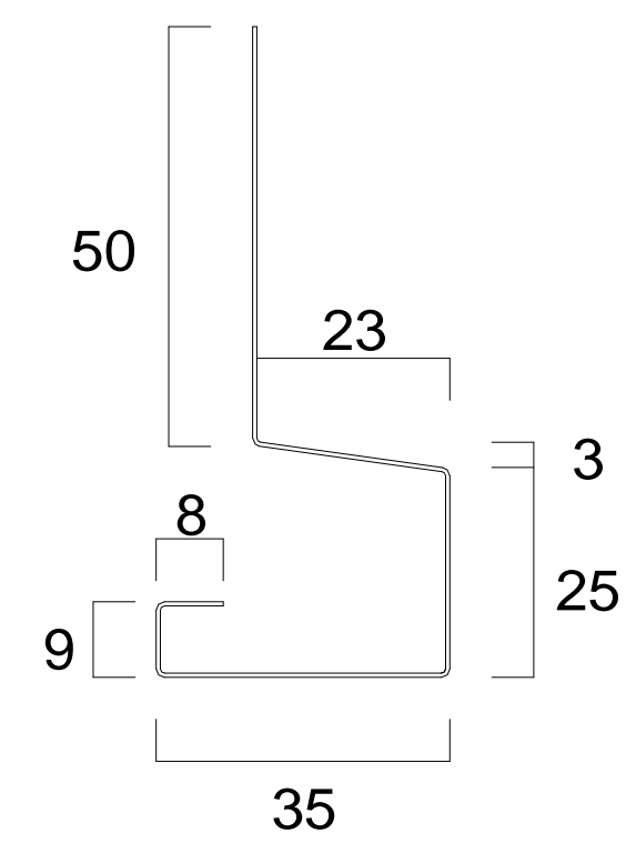
SP-201 (水切) L = 2000 ~ 3000
