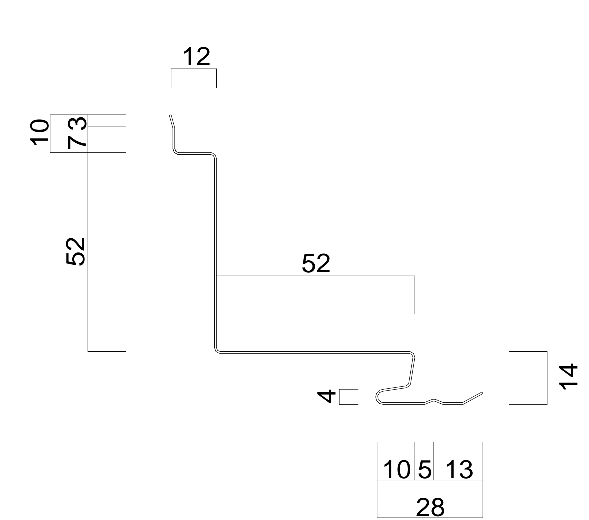
SPR105 (入隅) L = 2000 ~ 3000
