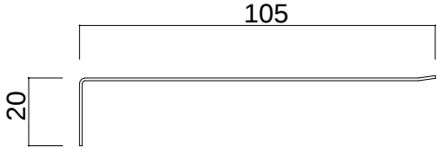
S U S - 2 B けらば力骨 t = 0 . 8
