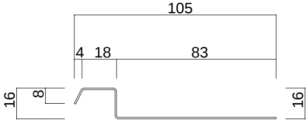
S U S - 2 B 軒先力骨（直葺用）t = 0 . 8
