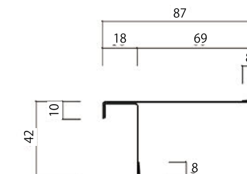
eルーフI型用ケラバ唐草ER-23
