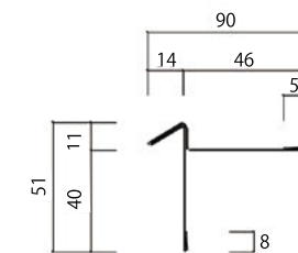
eルーフI型用ケラバ唐草ER-23
