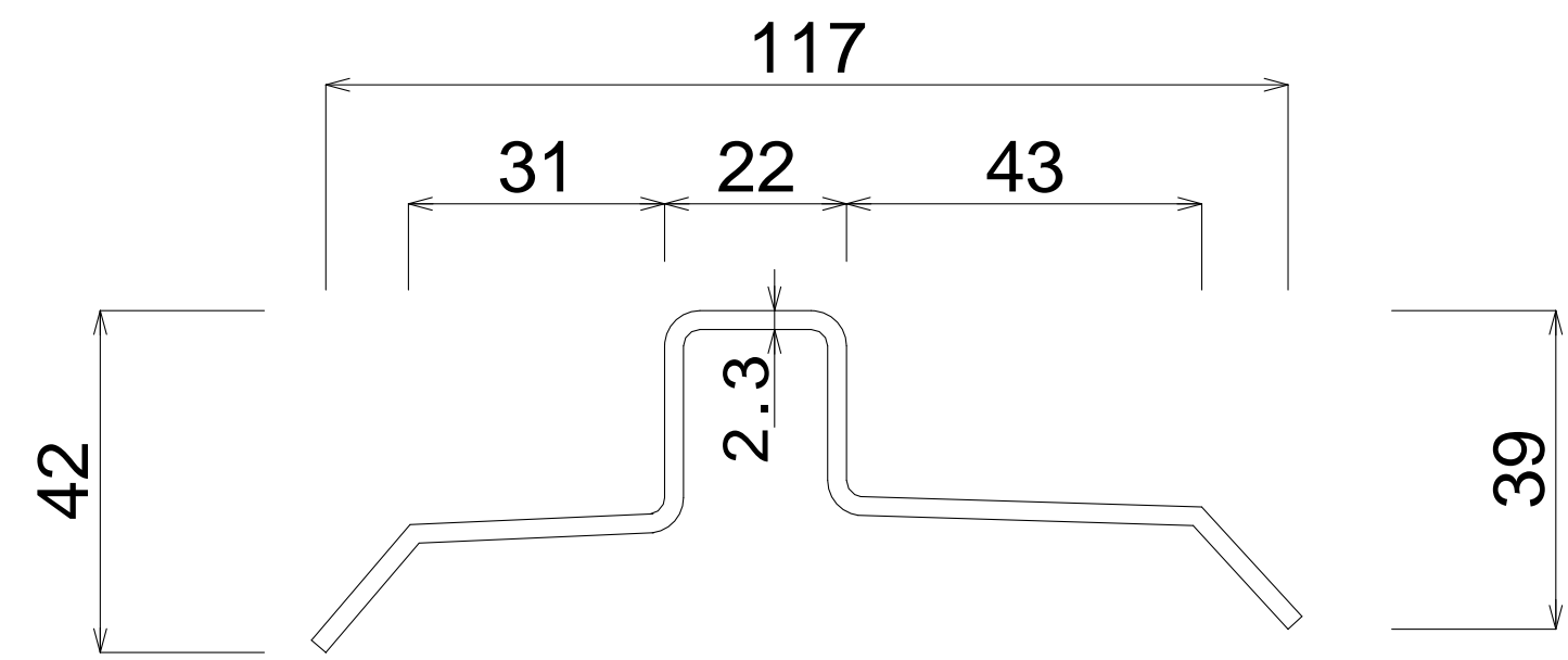
K R角ハゼ500 ( D 1 6 0 ) 吊子W = 30
