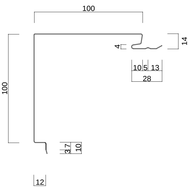
S P R 200 ( 出隅 ) L = 2 0 0 0 ~ 3 0 0 0
