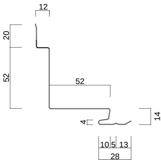
SPR116M (入隅) L = 2000 ~ 3000
