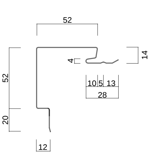
SPR116M (出隅) L = 2000 ~ 3000
