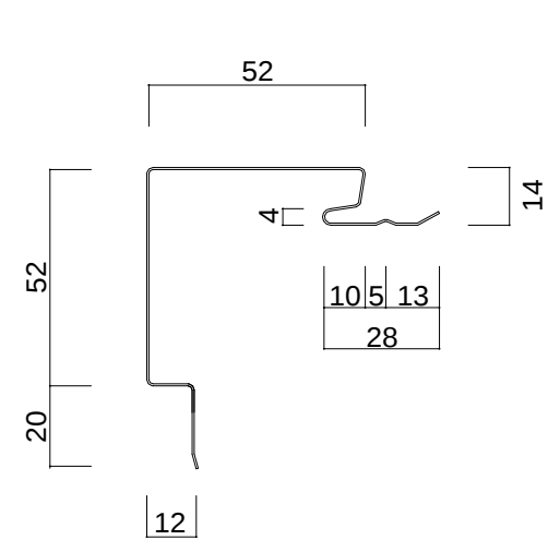
S P R 116 M ( 出隅 ) L = 2 0 0 0 ~ 3 0 0 0
