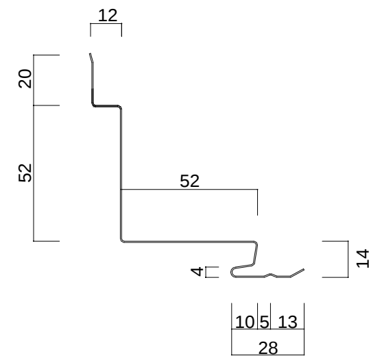
S P R 116 M ( 入隅 ) L = 2 0 0 0 ~ 3 0 0 0
