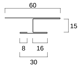
S P - 4 0 0 ( H型接続 ) L = 2 0 0 0 ~ 3 0 0 0
