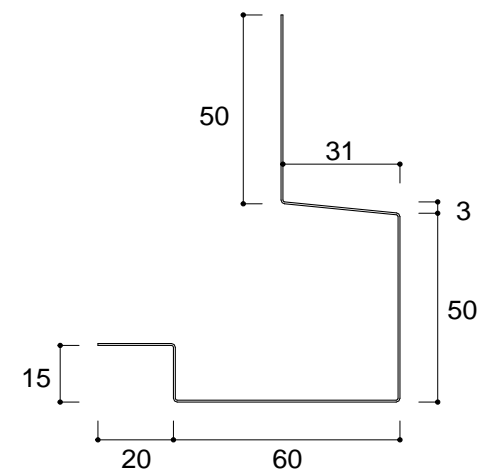
BK - 150 (天井見切水切) L = 2000 ~ 3000
